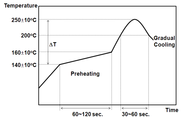
Infrared Reflow
